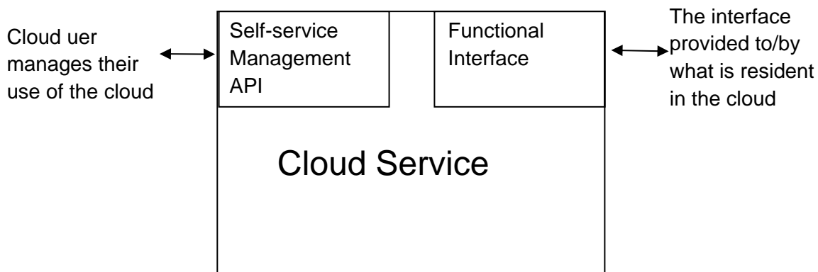
Figure 8 – Cloud Service Presents an Interface of Each Category
